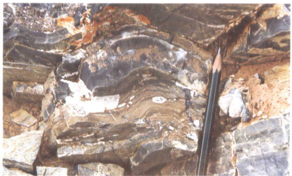
Figure 3-1: A photograph showing a geological rock face with distinct, wavy sedimentary layers. A black pencil is placed vertically against the rock to provide a scale for the thickness of the layers.
